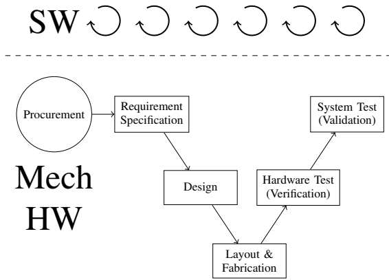
Fig. 1. Traditional mechanical/hardware and software co-design workflow
